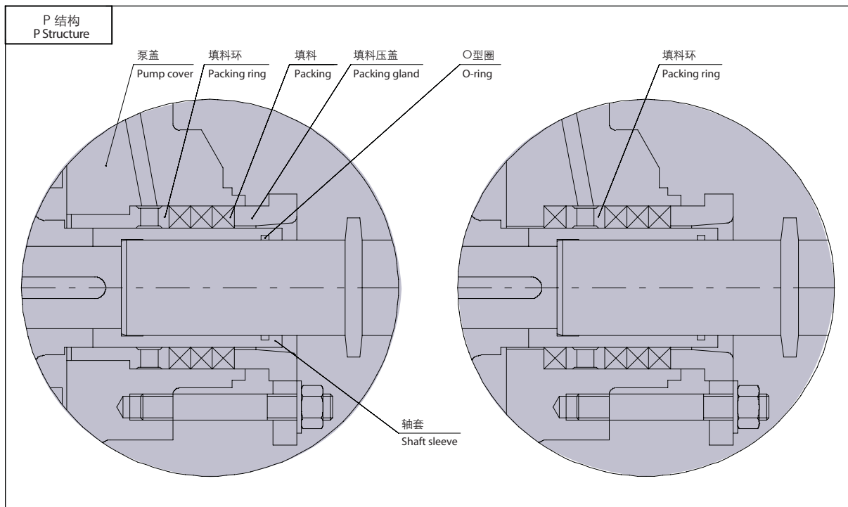
P结构: 外装式填料密封结构, 主要用于可容许少量泄漏之场所 P structure: outside-fitted packing seal structure, mainly used in the place with small leakage.
